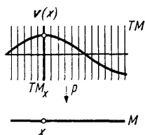
Fig. 257. A vector field
