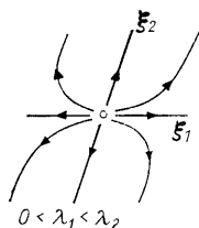
Fig. 135. An unstable node
