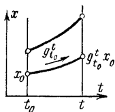
Fig. 70. The transformation over the time interval from t_0 to t
