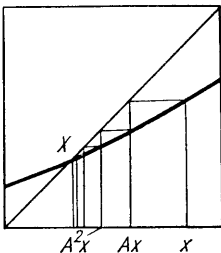
Fig. 212. The sequence of images of the point x under iteration of the contraction mapping A
