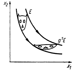
Fig. 47. A hyperbolic rotation
