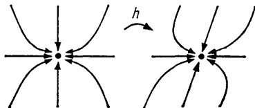
Fig. 150. Linearly equivalent systems
