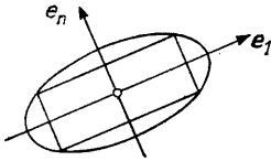
Fig. 180. The directions of the characteristic oscillations and the level lines of the potential energy
