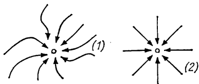
Fig. 167. The phase curves of Eqs. (1) and (2)
