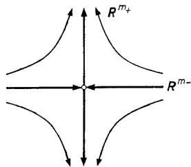
Fig. 162. The standard saddle point
