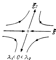
Fig. 134. A saddle point
