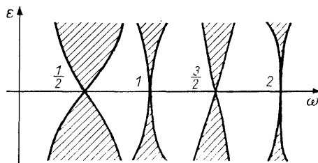
Fig. 209. The region of instability for Eq. (4)
