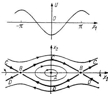
Fig. 106. The phase curves of the pendulum equation
