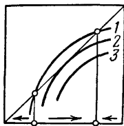
Fig. 36. Metamorphosis of Lamerey diagrams
