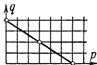
Fig. 68. The Newton diagram of a quasi-homogeneous function
