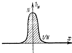
Fig. 44. A \delta -shaped sequence
