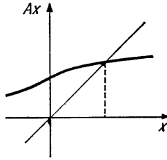
Fig. 211. The fixed point of a contraction mapping
