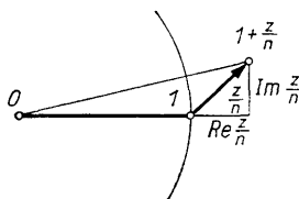
Fig. 110. The complex number 1 + (z/n)
