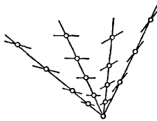
Fig. 63. The direction field of a homogeneous equation
