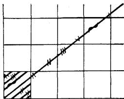
Fig. 175. An everywhere-dense curve on the torus
