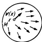
Fig. 257. A vector field
