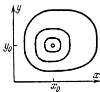
Fig. 34. The phase curves of the Lotka-Volterra model
