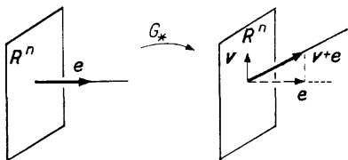
Fig. 229. The derivative of the mapping G at the point (t_0, x_0)
