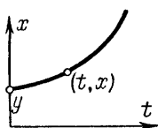
Fig. 59. Rectifying integral curves
