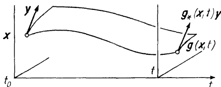
Fig. 227. The action of the transformation over the time from t_0 to t on a curve in the phase space and on a tangent vector to it
