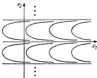
Fig. 60. A nonrectifiable direction field on the plane
