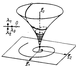
Fig. 146. The case \text{Re } \lambda_{1,2} < \lambda_3 < 0 . Contraction along the direction of \xi_3 , rotation with a more rapid contraction in the (\xi_1, \xi_2) -plane
