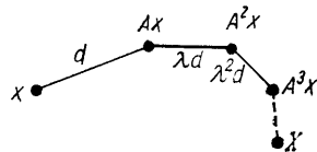
Fig. 213. An estimate of the accuracy of the approximation of x to the fixed point X
