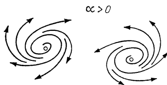
Fig. 138. Unstable foci
