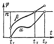
Fig. 202. Proof of the theorem on zeros
