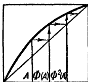
Fig. 19. The Lamerey staircase
