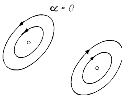
Fig. 137. Centers
