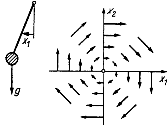
Fig. 22. The phase velocity field for small oscillations
