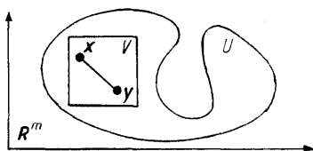
Fig. 220. Continuous differentiability implies a Lipschitz condition
