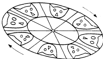
Fig. 132. An elliptic rotation
