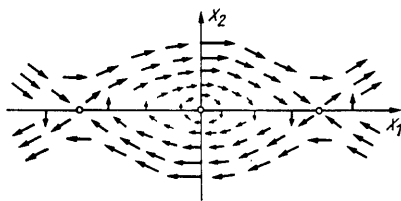
Fig. 24. The phase velocity field of the pendulum
