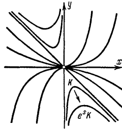
Fig. 65. The integral curves of a homogeneous equation
