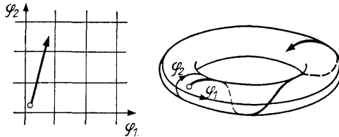
Fig. 174. A solenoid on the torus
