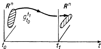
Fig. 196. The linear transformation of the phase space that is realized by the solutions of a linear equation over the time from t_0 to t_1
