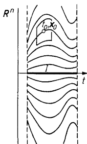
Fig. 191. The integral curves of a linear equation
