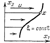
Fig. 75. Construction of rectifying coordinates
