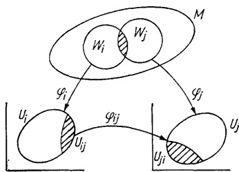
Fig. 233. Consistent charts
