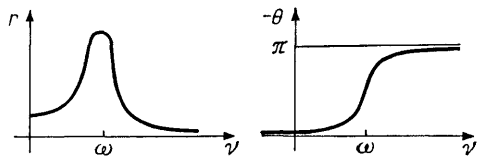
Fig. 188. The amplitude and phase of the forced oscillation of a pendulum with friction as a function of the frequency of the external force
