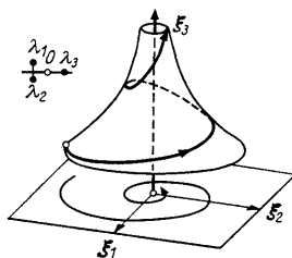
Fig. 148. The case \text{Re } \lambda_{1,2} < 0 < \lambda_3 . Dilation along the direction of \xi_3 , rotation with contraction in the (\xi_1, \xi_2) -plane
