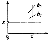
Fig. 223. Comparison of v_1 and v_2 .
