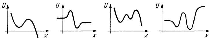
Fig. 96. Sketch the level lines of the energy
