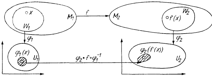
Fig. 242. A differentiable mapping
