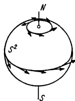
Fig. 258. A velocity field
