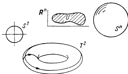
Fig. 231. Examples of manifolds
