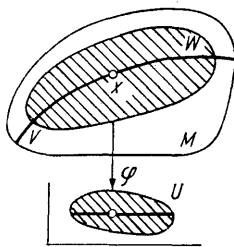
Fig. 246. A submanifold
