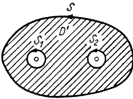
Fig. 270. A domain to which Green's formula applies
