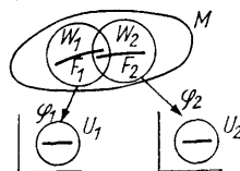
Fig. 240. A compact subset
