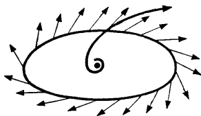
Fig. 155. The level surface of a Lyapunov function
