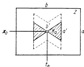
Fig. 221. The cylinder \mathcal{C} and the cone K_0
